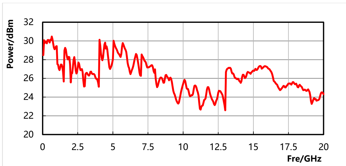
S1466D-V Max.output power measured value (High power option H05-20)
