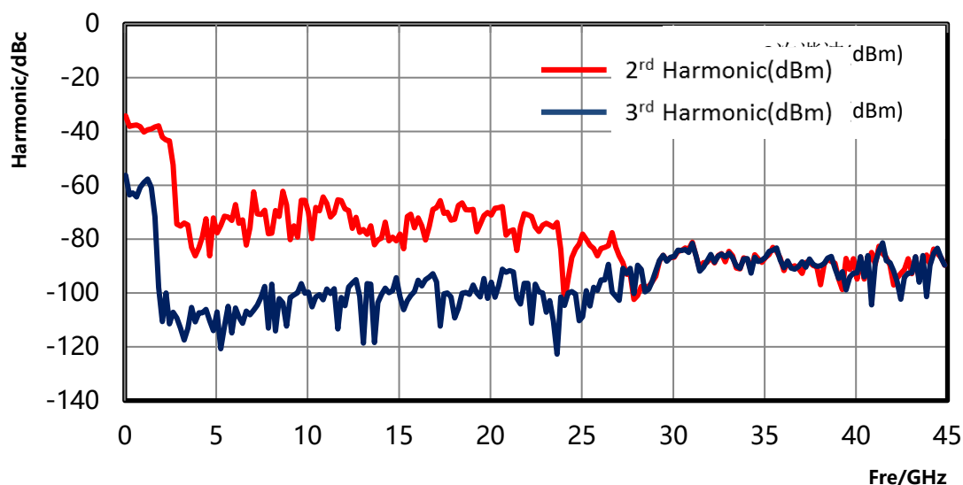
S1466G-V Harmonic measured value
