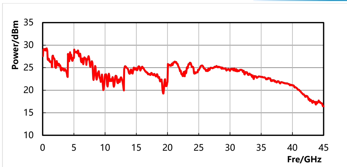
S1466G-V Max.output power measured value (High power option H05-45)
