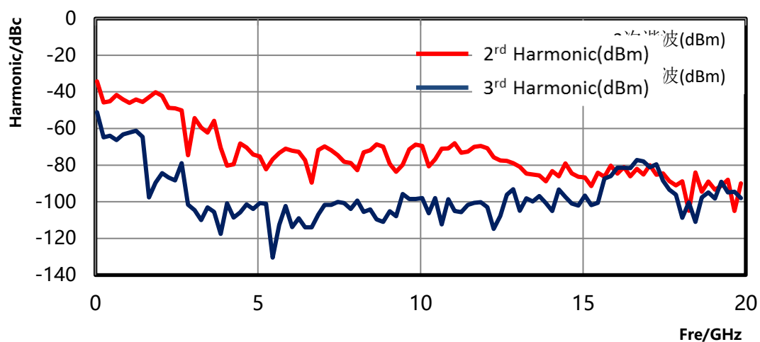
S1466D-V Harmonic measured value
