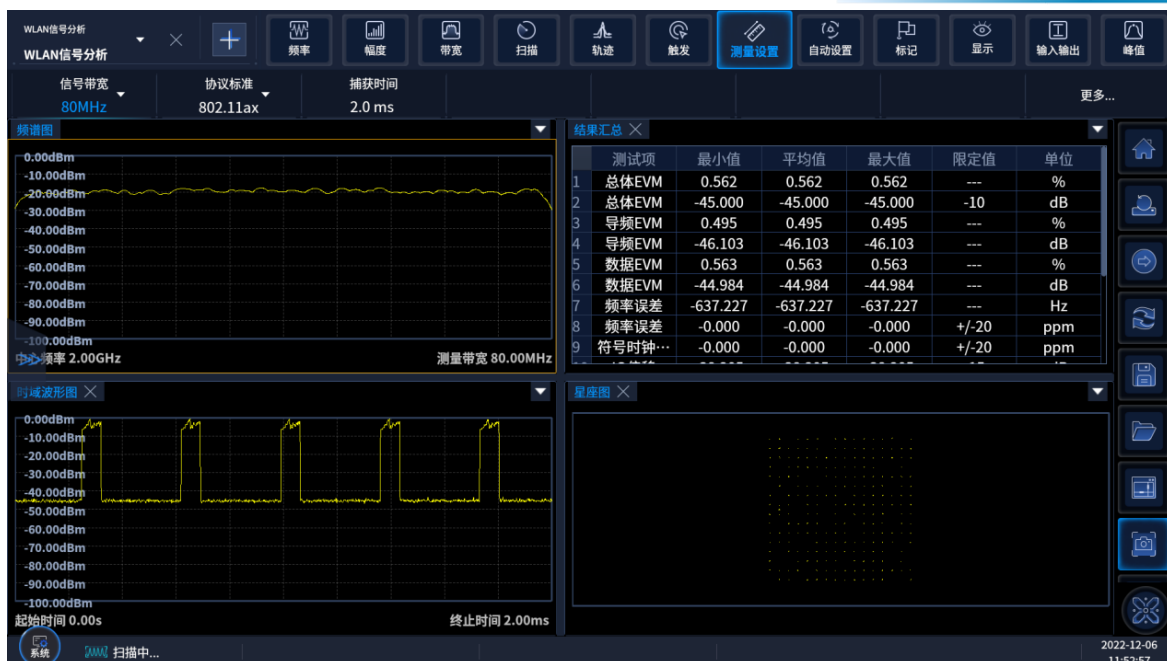
IEEE 802.11ax single user PPDU signal demodulation EVM 80MHz transmission bandwidth, 256QAM
