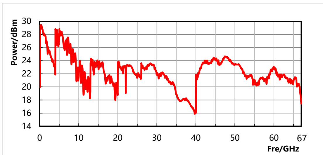
S1466L-V Max.output power measured value (High power option H05-67)
