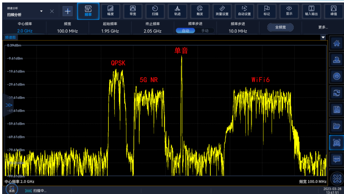
Different modulation types of multi-carrier test map
