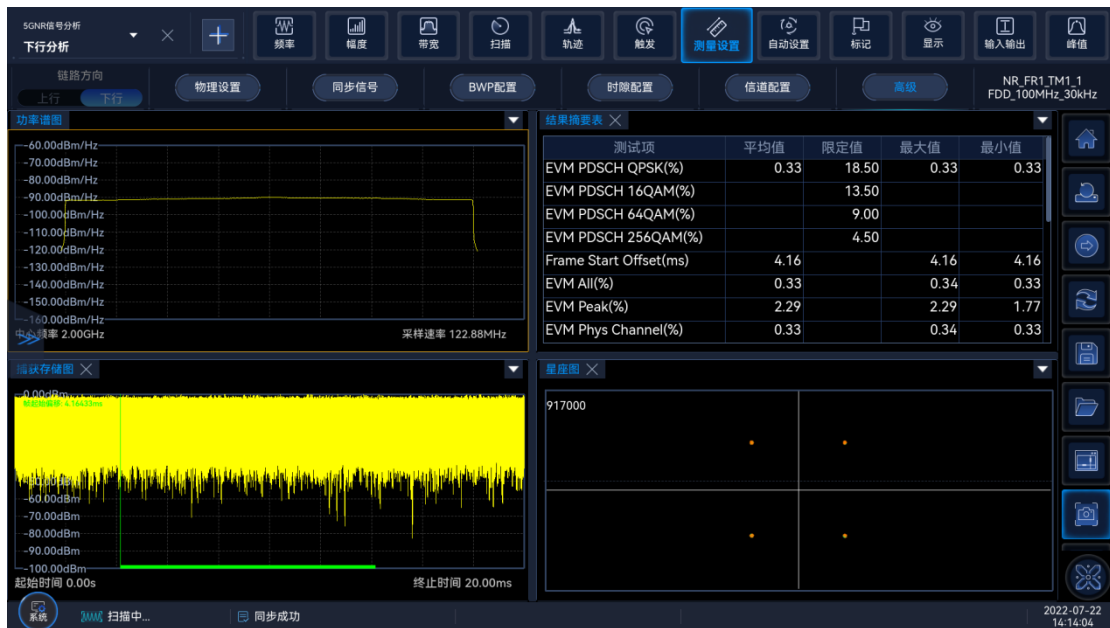
FR1-TM1_1_FDD_100MHz_30kHz measured value
