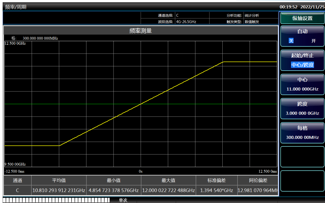
Analog sweep (ramp sweep) measured value
