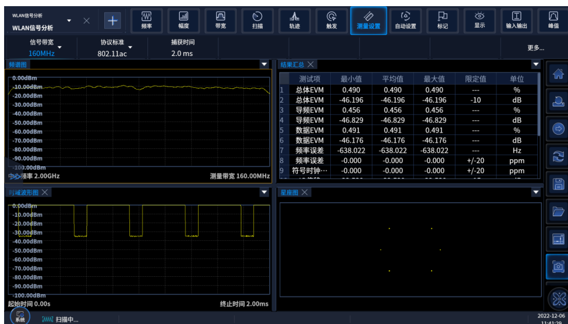
IEEE 802.11ac single user PPDU signal demodulation EVM 160MHz transmission bandwidth, QPSK+BPSK
