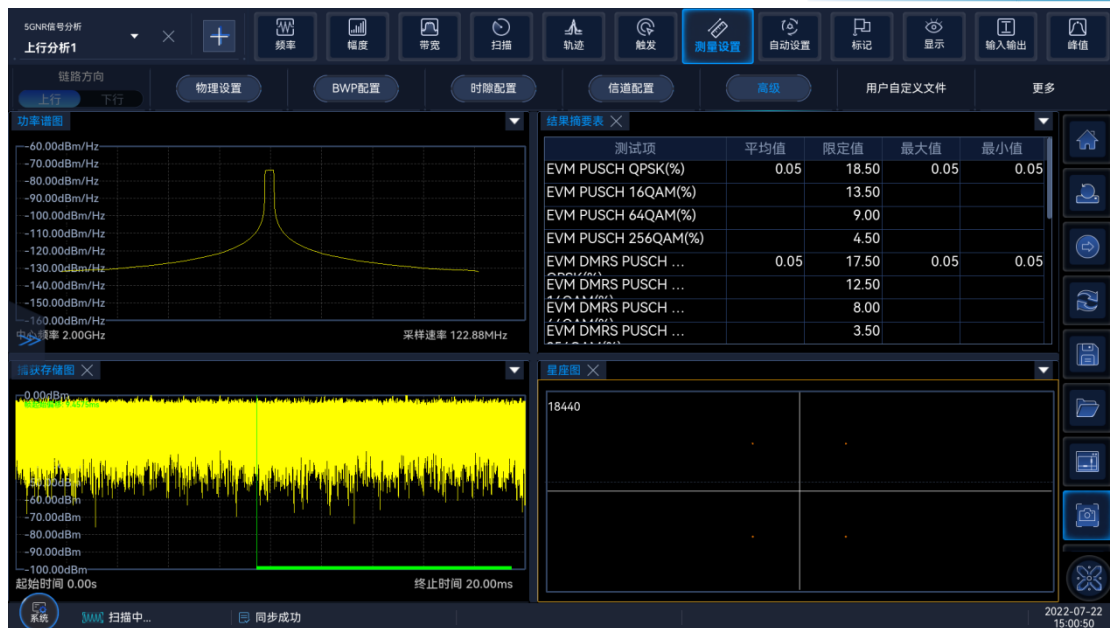
FRC-FR1-100MHz_A1-8 measured value
