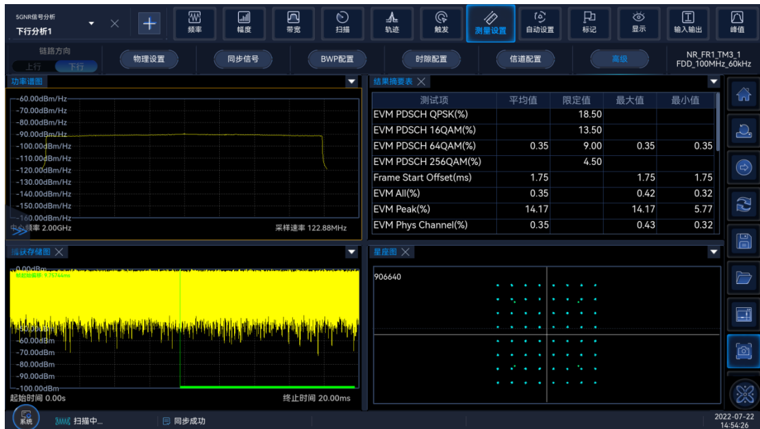
FR1-TM3_1_FDD_100MHz_60kHz measured value
