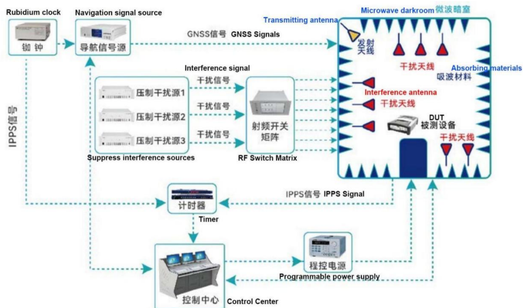
Satellite Navigation Wireless Test System
