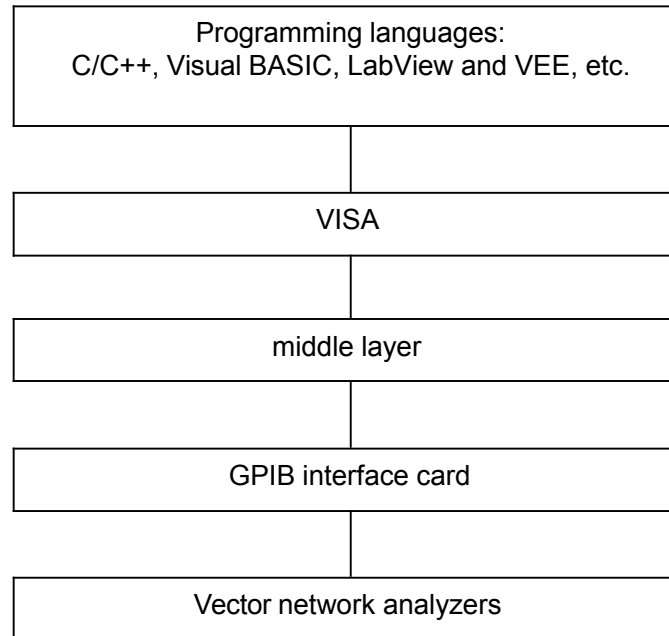
Figure 1-1 Software/hardware Layers
