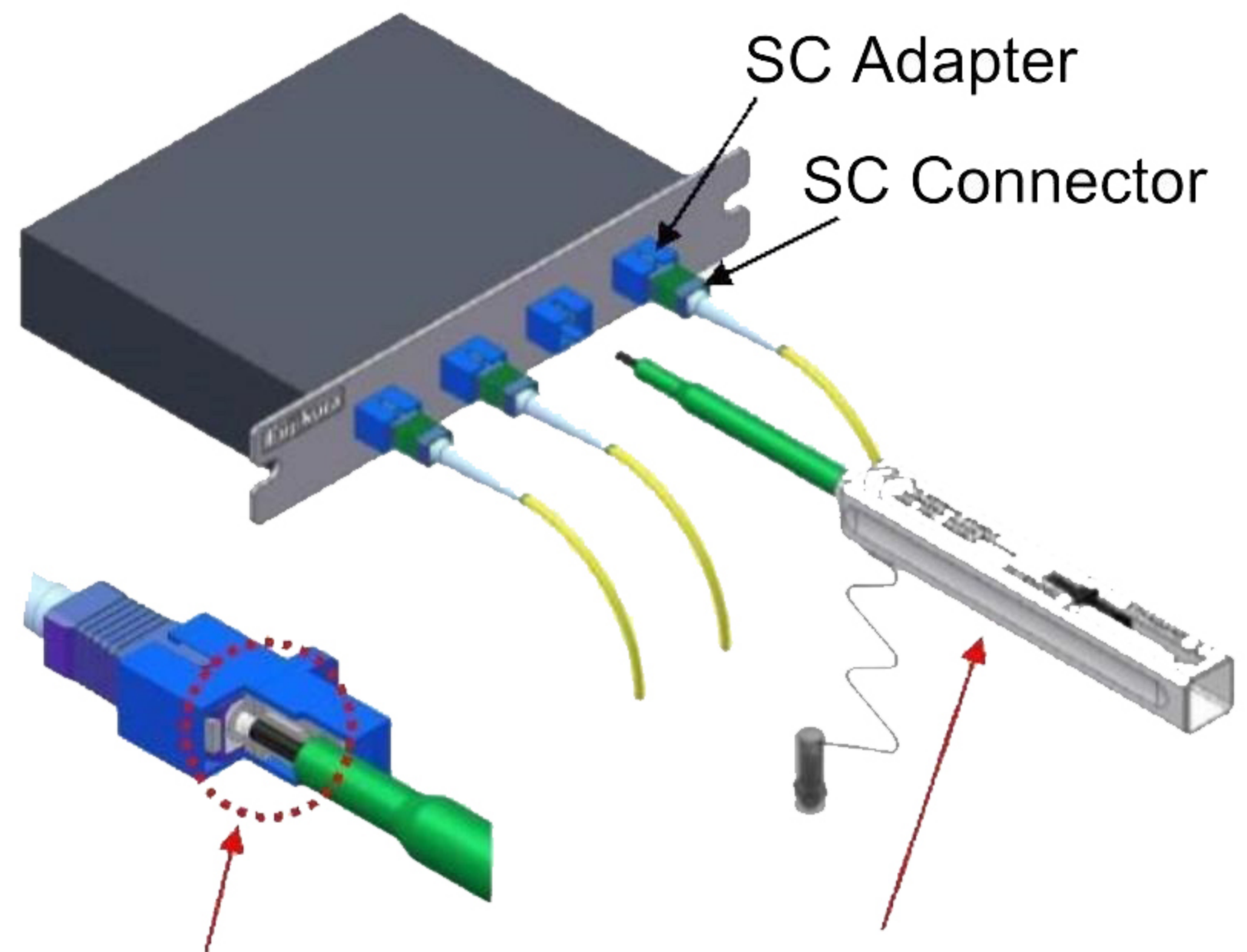
One-Click Cleaner 2.5mm
