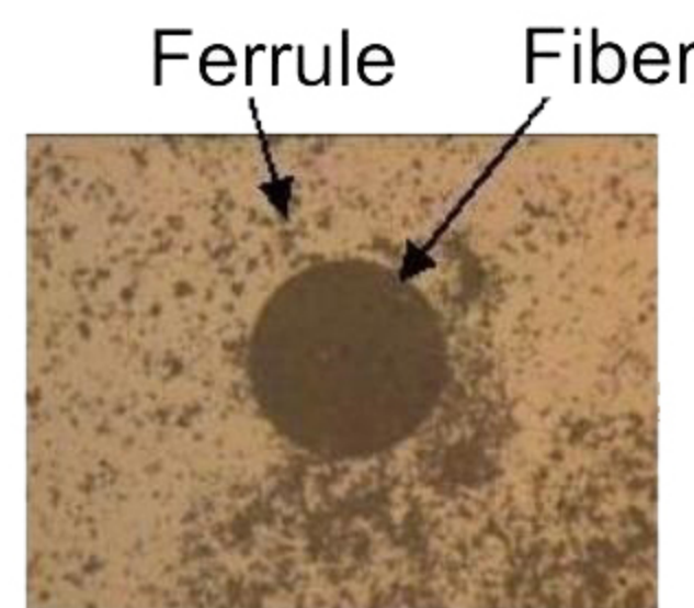
Before Cleaning
