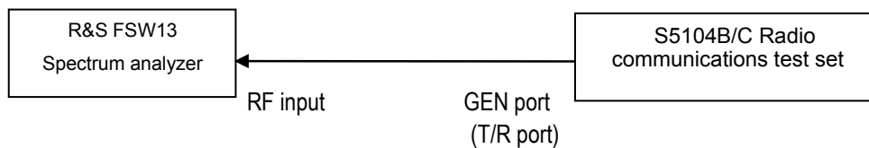
Fig. 6-1 Block diagram for RF signal generation characteristics test
