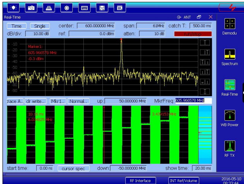
Fig. 3-11 Real-time spectrum analysis interface
