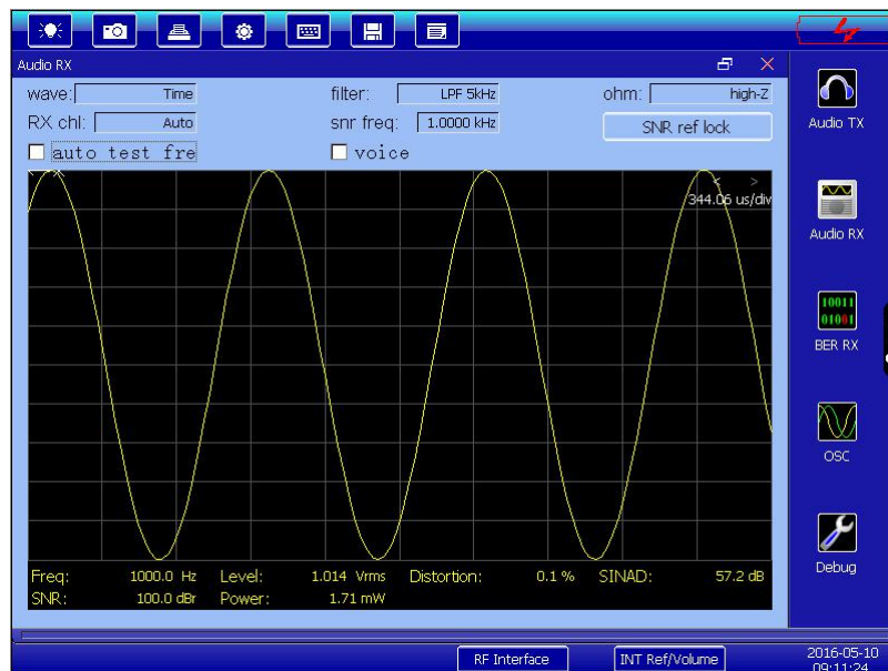
Fig.4-15 Audio analysis results
