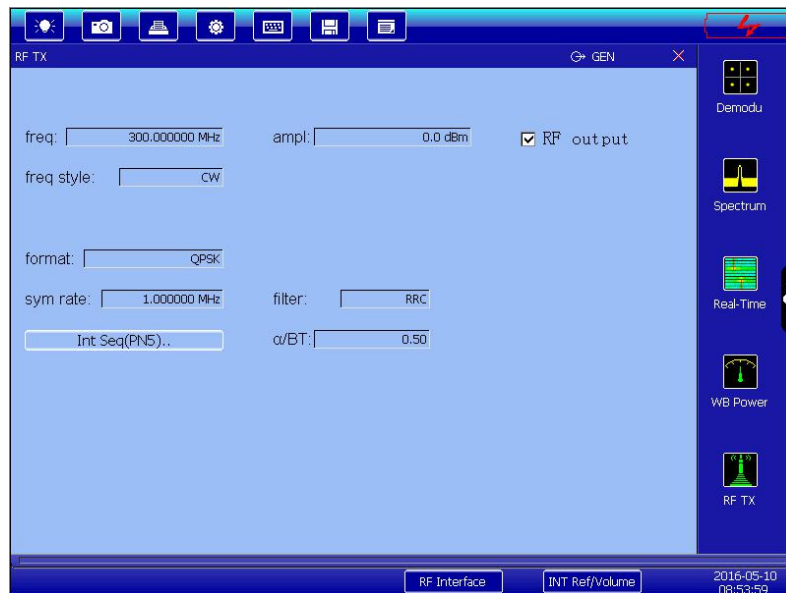
Fig. 4-3 Digital modulation signal output interface
