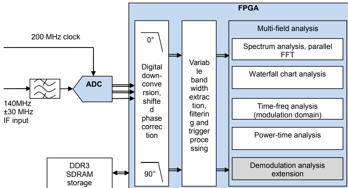
Fig.5-6 Block diagram of receiver IF digital signal processing
