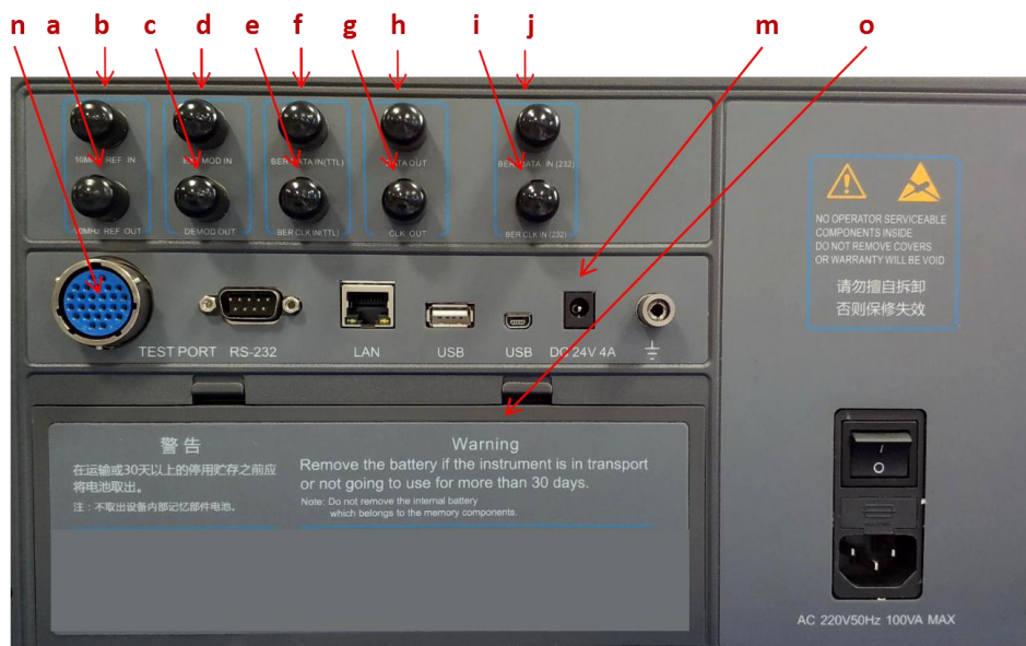
Fig. 2-3 Rear panel schematic diagram of the S5104 series radio communications test set
