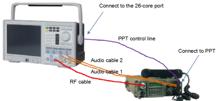
Fig.4-21 Typical one-click auto test connection diagram
