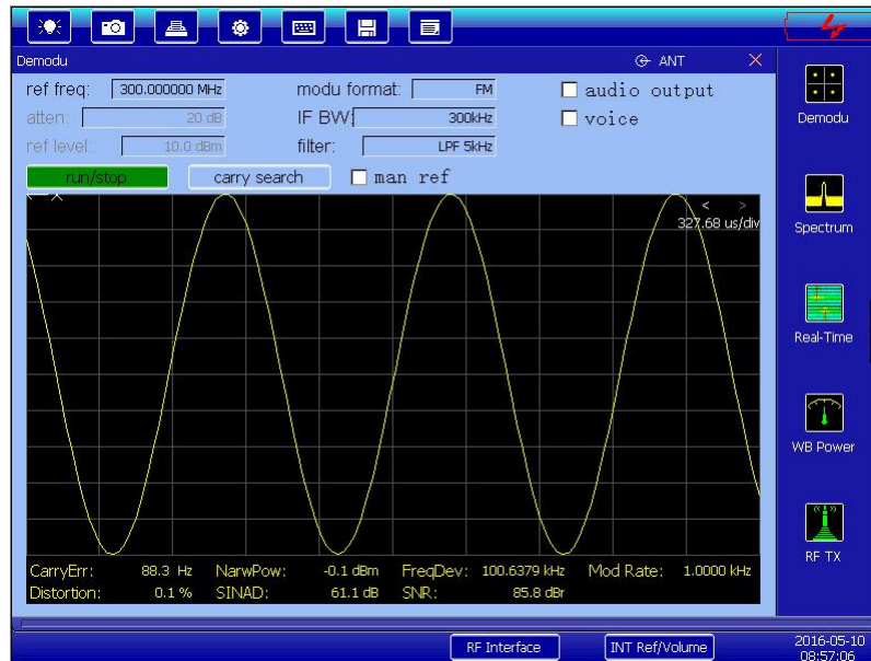
Fig. 4-6 FM demodulation interface
