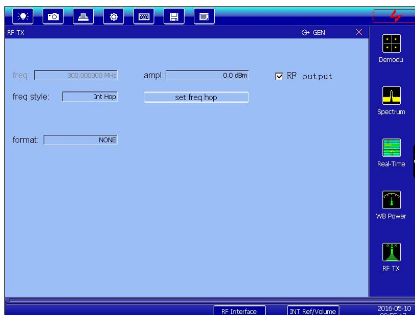
Fig. 4-4 Frequency hopping signal output interface
