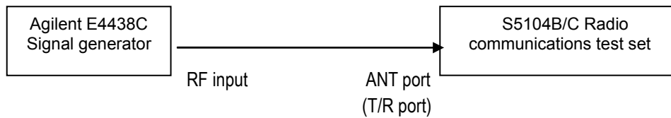
Fig. 6-2 Block diagram for RF RX and sweep spectrum characteristics tests
