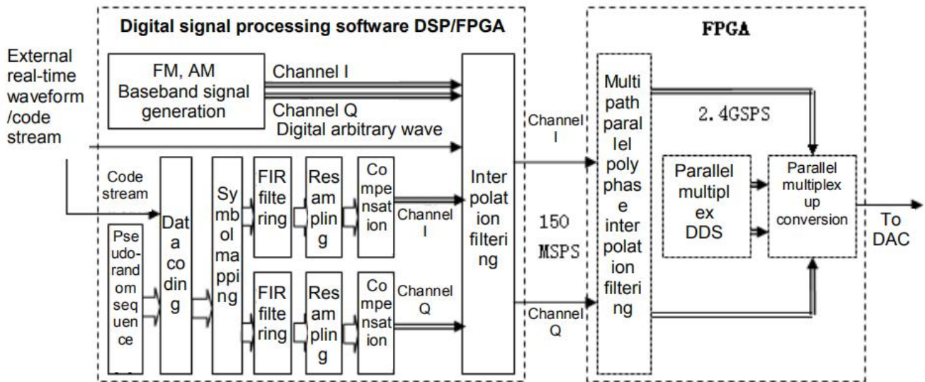
Fig.5-7 Block diagram of transmitter IF digital signal processing
