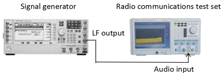
Fig.4-14 Audio analyzer connection diagram
