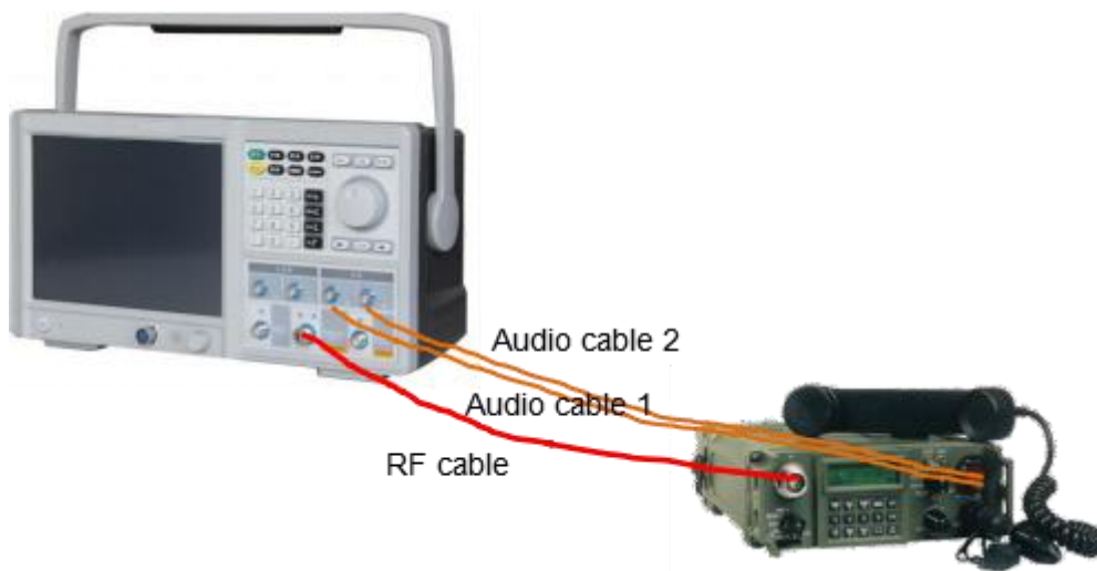
Fig.4.-20 Typical auto test connection diagram
