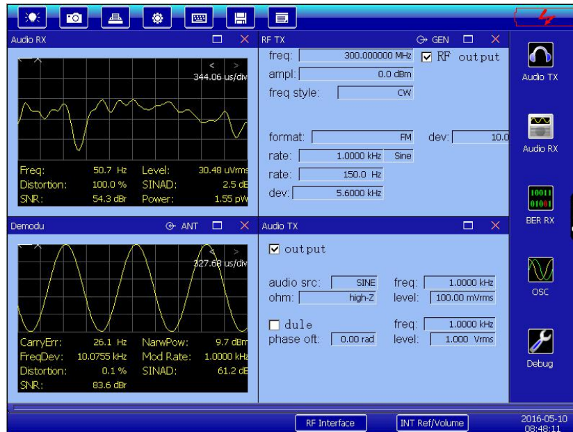
Fig. 3-19 Combined interface: RF emission, RF receipt, audio generation and audio analysis 13: Auto test:
