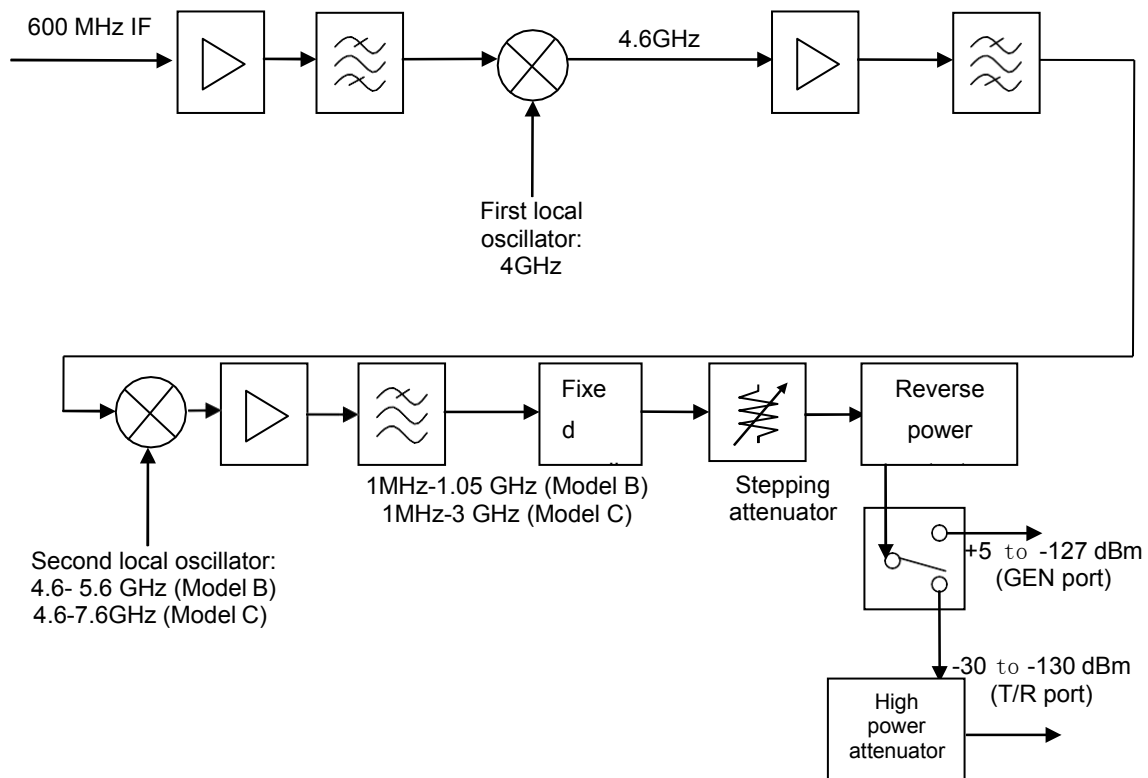
Fig.5-3 RF conversion scheme of the transmitter
