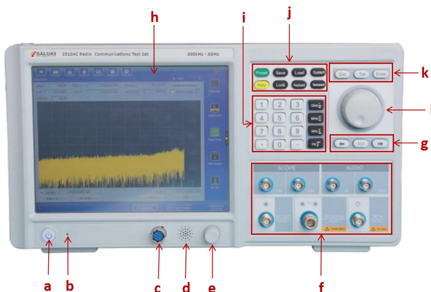
Fig.2-2 Front panel schematic diagram of the S5104 series radio communications test set
