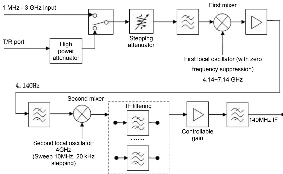
Fig. 5-4 RF conversion scheme of the receiver
