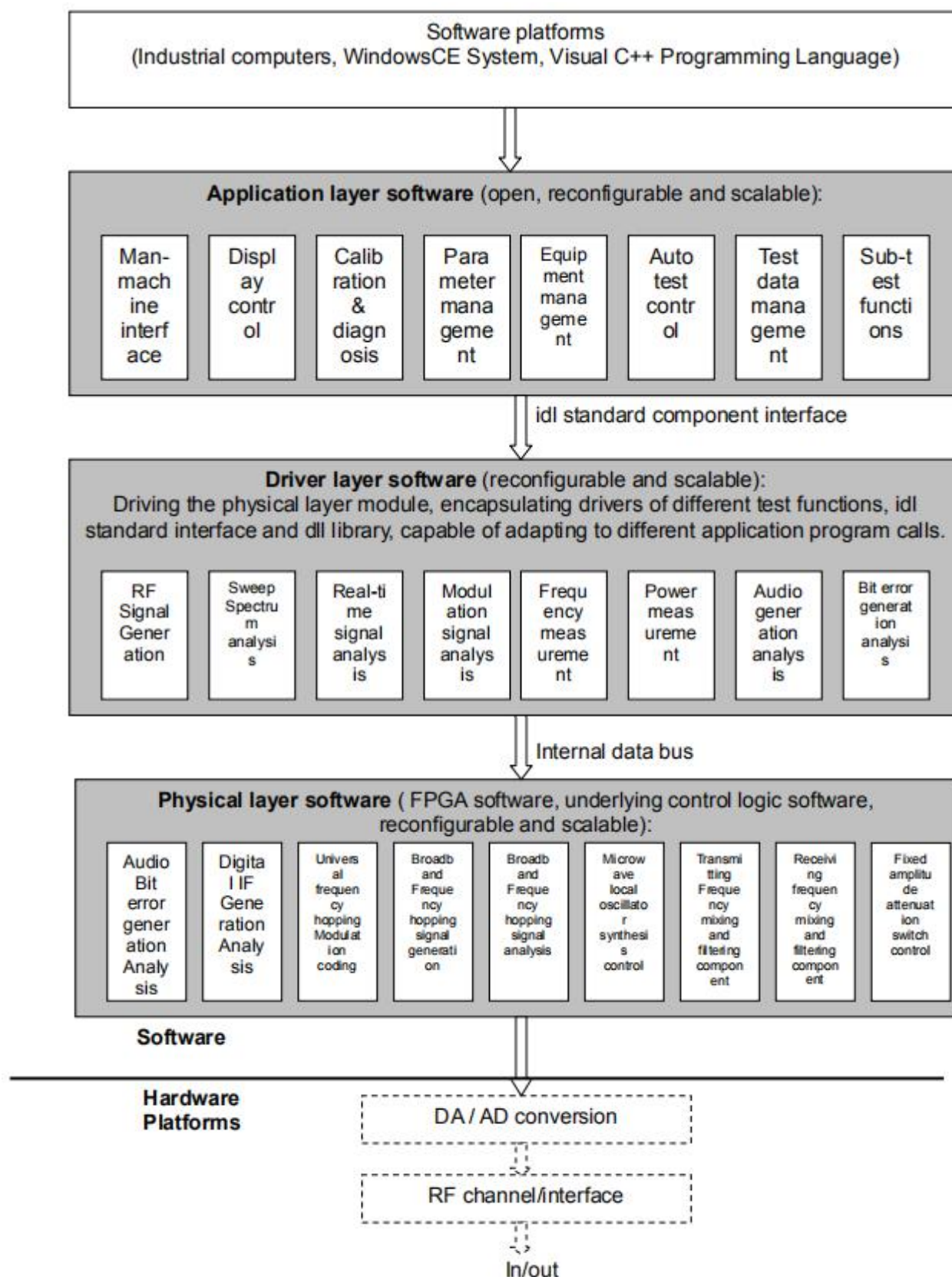
Fig. 5 -2 Overall software solution based on software radio
