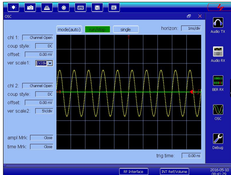
Fig.4-18 Oscilloscope test result
