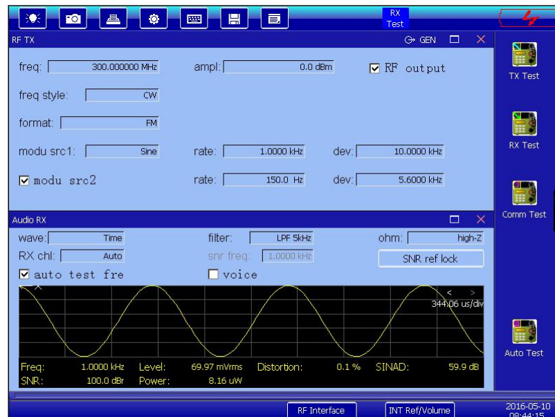
Fig. 3-17 Combined interface: RF emission and audio analysis
