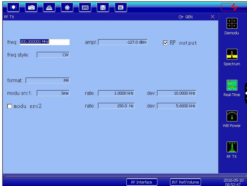
Fig.4-2 FM signal output interface
