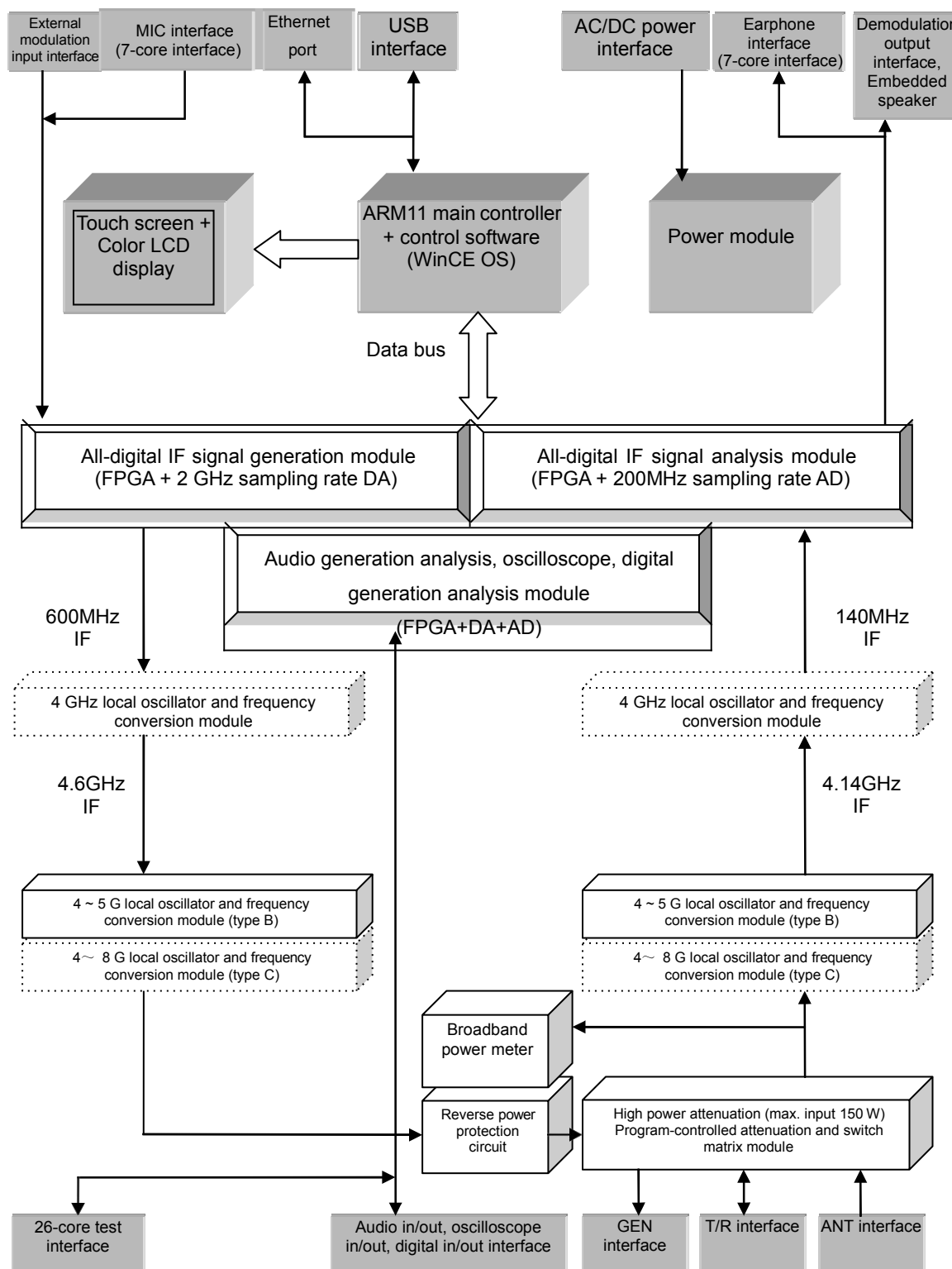
Fig.5-1 Hardware block diagram of S5104 series radio communications test set
