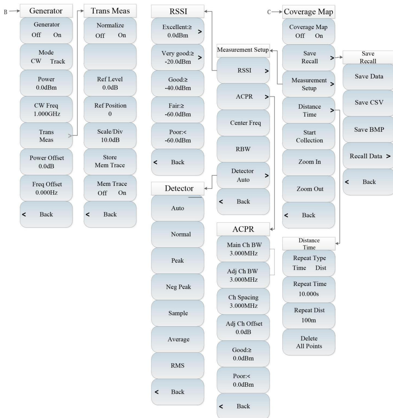
Fig. 4-33 Overall Block Diagram of Spectrum Analysis Menu (continued)
