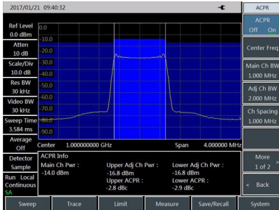
Fig. 4-4 ACPR Measurement
