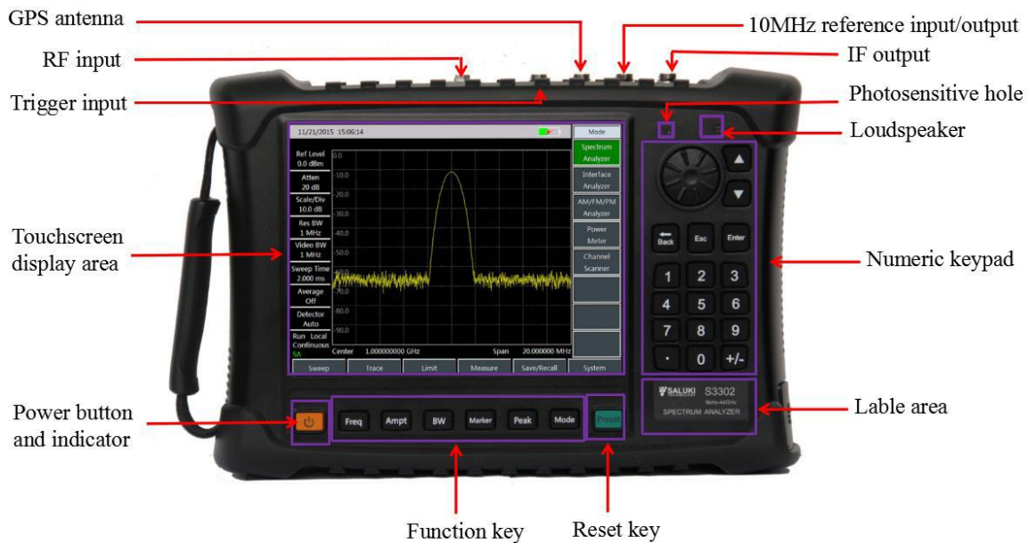
Fig. 3-1 Front Panel
